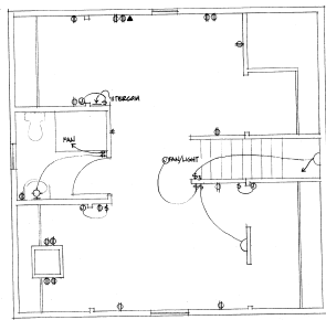
3 RD FLOOR ELECTRICAL PLAN 18'-11" x 17'
