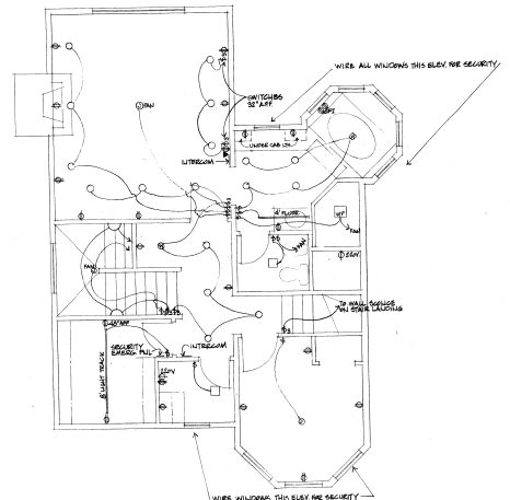
2 ND FLOOR ELECTRICAL PLAN 18'-11" x 17'
